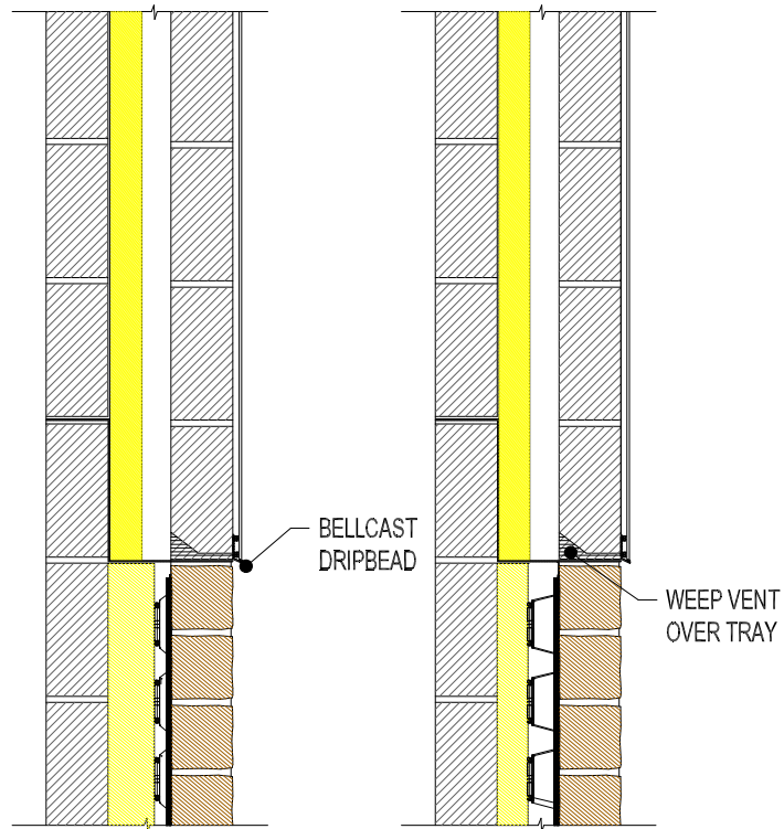
SURECAV25 SURECAV25 WITH 75mm INSULATION BELOW THE TRAY AND 50mm ABOVE
